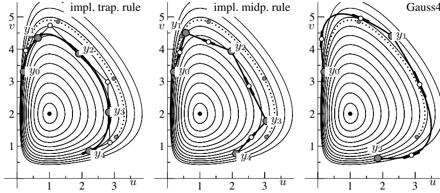
Fig. 1.3. Collocation solutions for the Lotka–Volterra problem (I.1.1); u_0 = 0.2 , v_0 = 3.3 ; methods of order 2: four steps with h = 0.4 ; method of order 4: two steps with h = 0.8 ; dotted: exact solution
